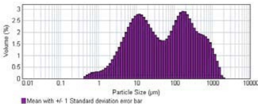
FIGURE 1 BIMODAL GRAIN SIZE DISTRIBUTION OF SEDIMENT WITHIN WRECK B125/306B, SAMPLE 2A 30/07/2008 © MASTERSIZER2000
