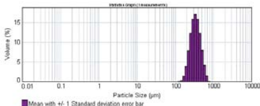
FIGURE 2 UNIMODAL GRAIN SIZE DISTRIBUTION OF SEDIMENT OUTSIDE T-319 B112/238 WRECK, SAMPLE B 20/03/2009 © MASTERSIZER2000
