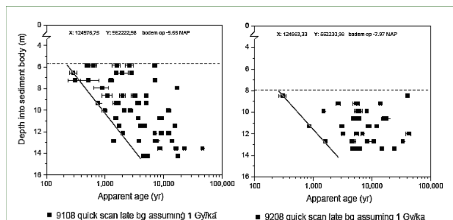
FIGURE 5 Preliminary OSL age estimates using 'quick and dirty' methods. Note that the results are too scattered to convincingly guide sample selection for full OSL analysis.
